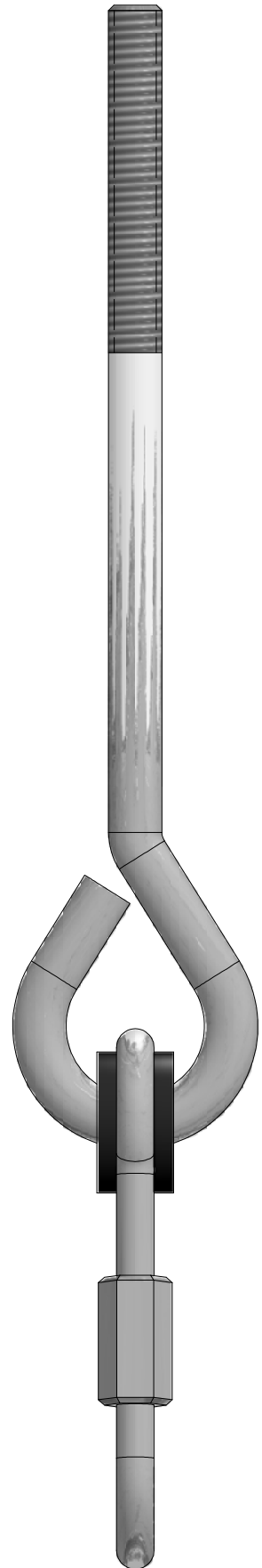
(4) BZ - SWING HANGER QUICK LINK - H100099
